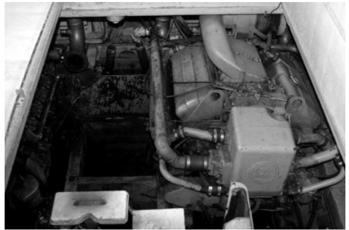
POWERED BY GM DETROIT 8V-53 ENGINES WITH TWIN DISC MG 506 GEARS
